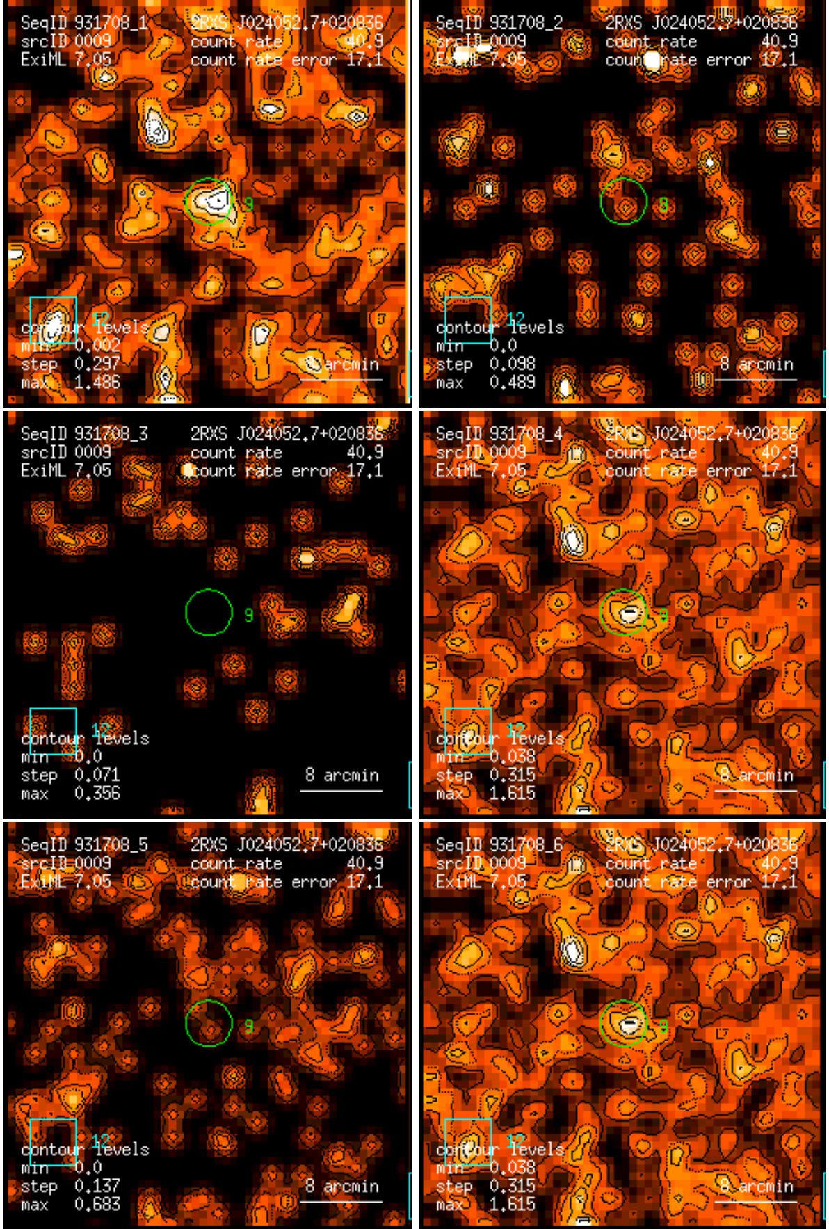
Figure 9: RASS 931708: detection 0009: band rate images, Gaussian filter: (1) PSPC channels 11 – 41, (2) 52 – 90, (3) 91 – 201, (4) 11 – 235, (5) 52 – 201, (6) 11 – 201. Broad band rates in counts/ks. Band rate contour levels in counts/ks/arcmin 2 .
