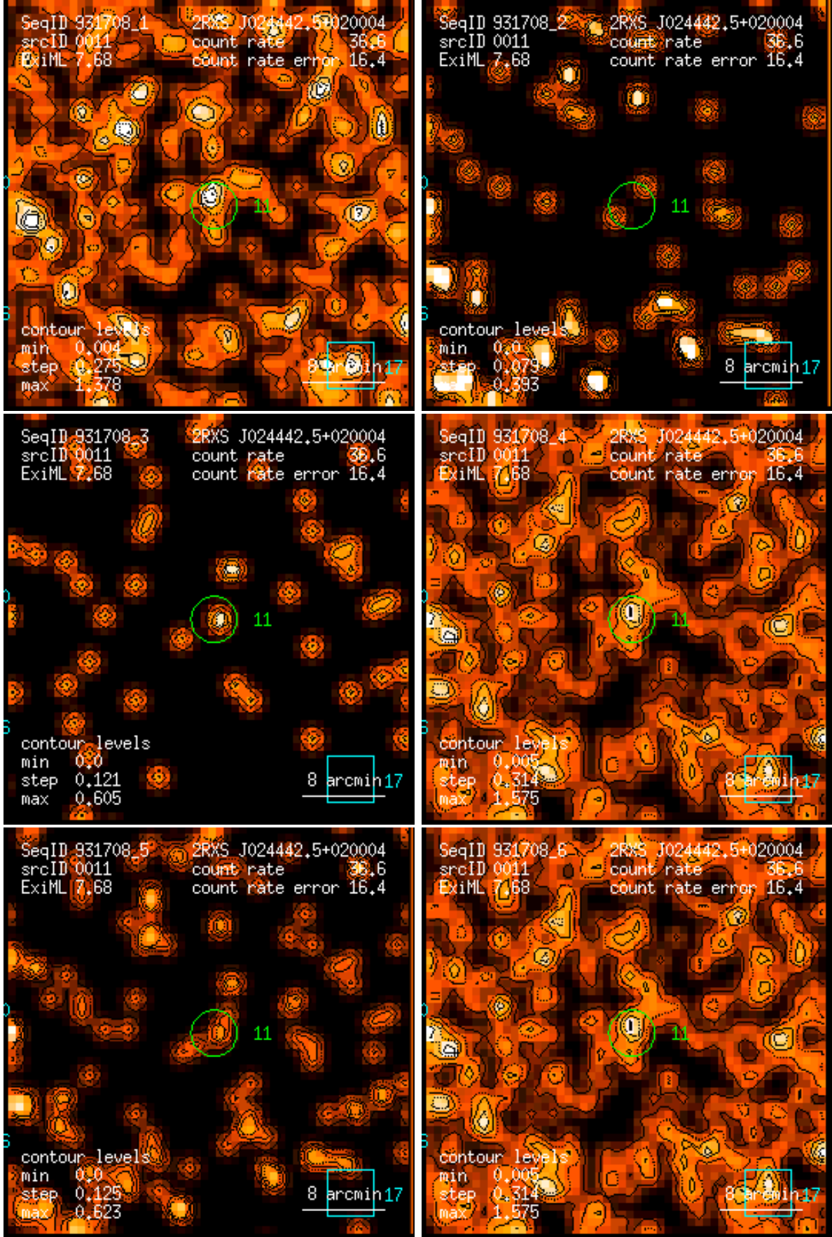
Figure 11: RASS 931708: detection 0011: band rate images, Gaussian filter: (1) PSPC channels 11 – 41, (2) 52 – 90, (3) 91 – 201, (4) 11 – 235, (5) 52 – 201, (6) 11 – 201. Broad band rates in counts/ks. Band rate contour levels in counts/ks/arcmin 2 .
