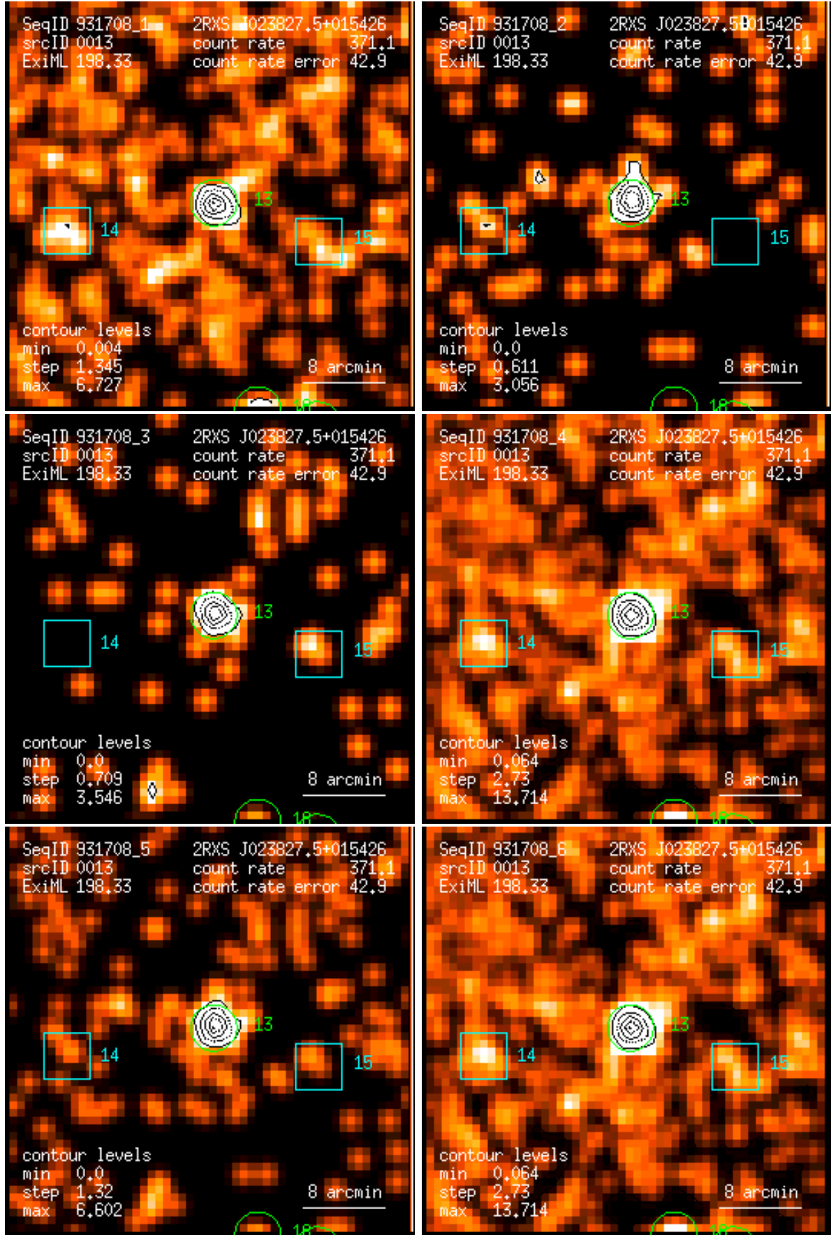
Figure 13: RASS 931708: detection 0013: band rate images, Gaussian filter: (1) PSPC channels 11 – 41, (2) 52 – 90, (3) 91 – 201, (4) 11 – 235, (5) 52 – 201, (6) 11 – 201. Broad band rates in counts/ks. Band rate contour levels in counts/ks/arcmin 2 .
