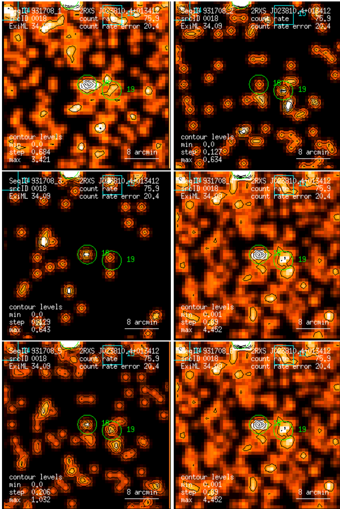
Figure 18: RASS 931708: detection 0018: band rate images, Gaussian filter: (1) PSPC channels 11 – 41, (2) 52 – 90, (3) 91 – 201, (4) 11 – 235, (5) 52 – 201, (6) 11 – 201. Broad band rates in counts/ks. Band rate contour levels in counts/ks/arcmin 2 .
