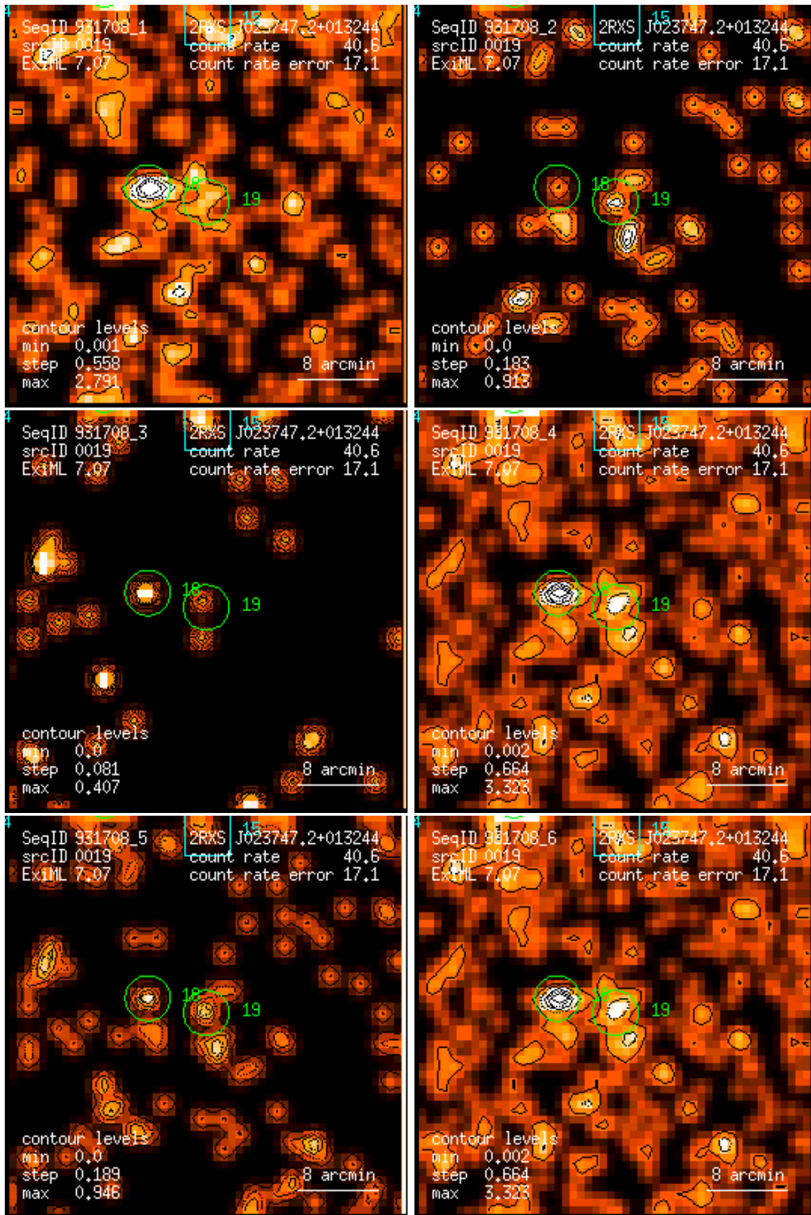
Figure 19: RASS 931708: detection 0019: band rate images, Gaussian filter: (1) PSPC channels 11 – 41, (2) 52 – 90, (3) 91 – 201, (4) 11 – 235, (5) 52 – 201, (6) 11 – 201. Broad band rates in counts/ks. Band rate contour levels in counts/ks/arcmin 2 .
