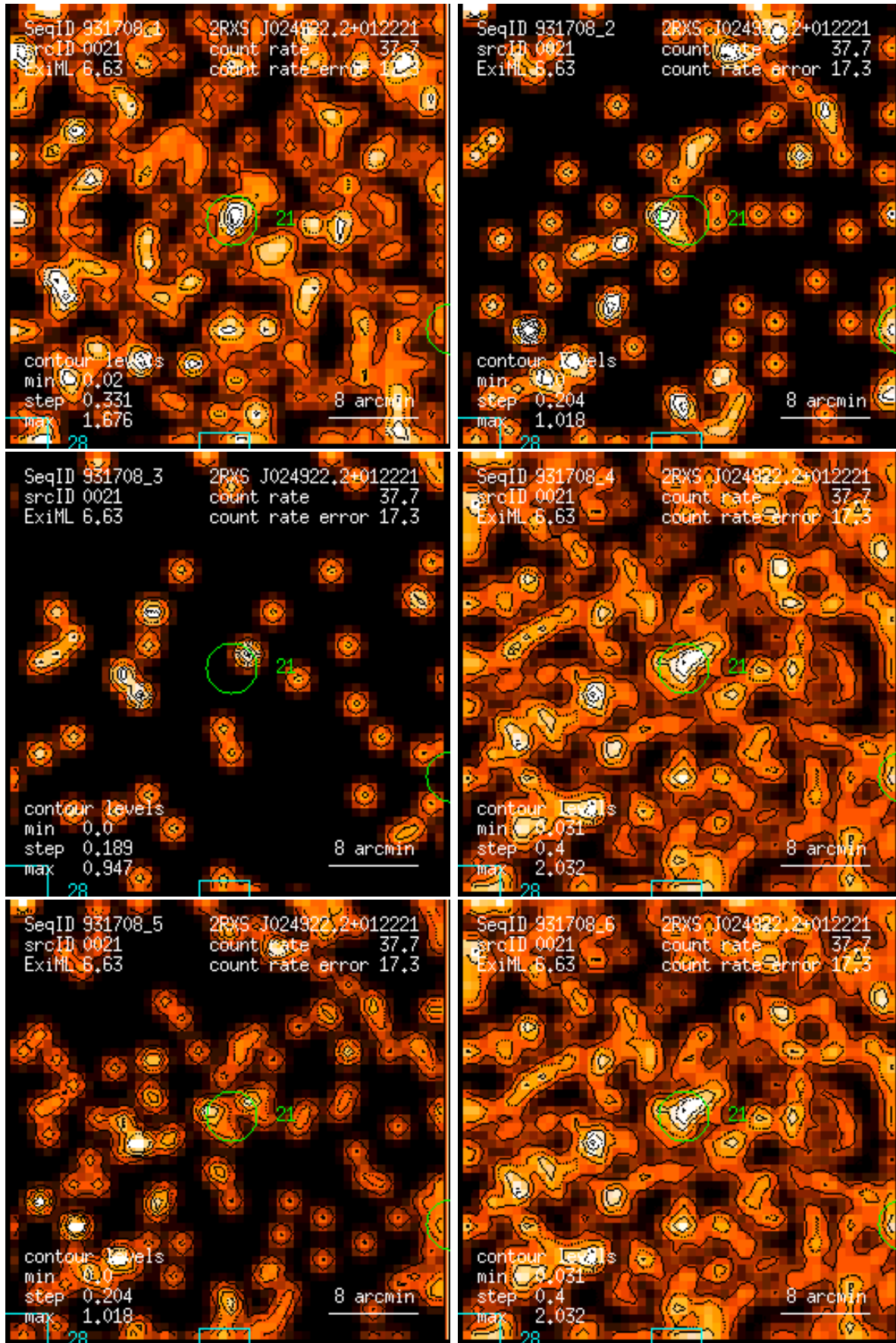
Figure 21: RASS 931708: detection 0021: band rate images, Gaussian filter: (1) PSPC channels 11 – 41, (2) 52 – 90, (3) 91 – 201, (4) 11 – 235, (5) 52 – 201, (6) 11 – 201. Broad band rates in counts/ks. Band rate contour levels in counts/ks/arcmin 2 .
