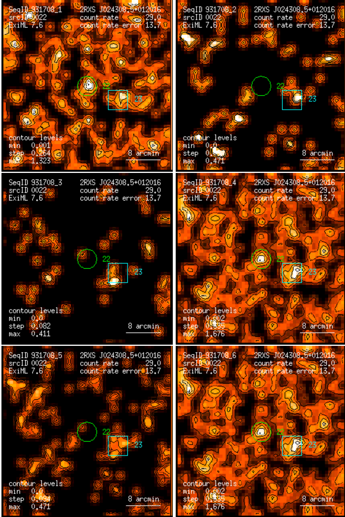
Figure 22: RASS 931708: detection 0022: band rate images, Gaussian filter: (1) PSPC channels 11 – 41, (2) 52 – 90, (3) 91 – 201, (4) 11 – 235, (5) 52 – 201, (6) 11 – 201. Broad band rates in counts/ks. Band rate contour levels in counts/ks/arcmin 2 .
