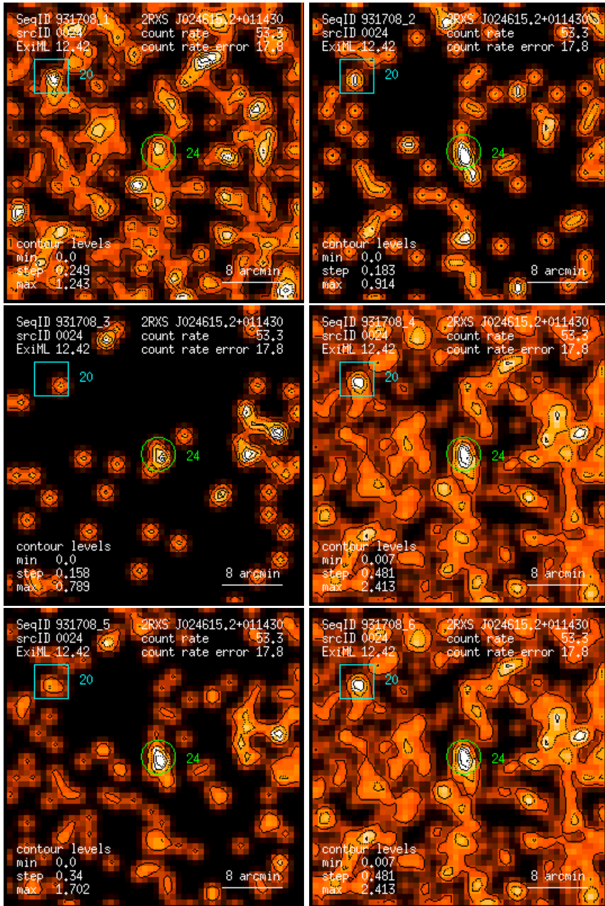
Figure 24: RASS 931708: detection 0024: band rate images, Gaussian filter: (1) PSPC channels 11 – 41, (2) 52 – 90, (3) 91 – 201, (4) 11 – 235, (5) 52 – 201, (6) 11 – 201. Broad band rates in counts/ks. Band rate contour levels in counts/ks/arcmin 2 .
