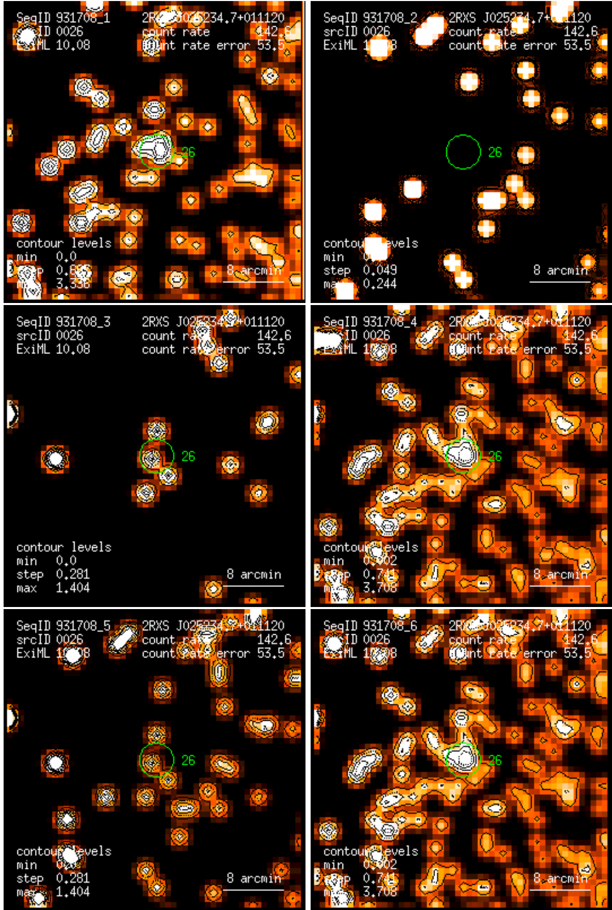
Figure 26: RASS 931708: detection 0026: band rate images, Gaussian filter: (1) PSPC channels 11 – 41, (2) 52 – 90, (3) 91 – 201, (4) 11 – 235, (5) 52 – 201, (6) 11 – 201. Broad band rates in counts/ks. Band rate contour levels in counts/ks/arcmin 2 .
