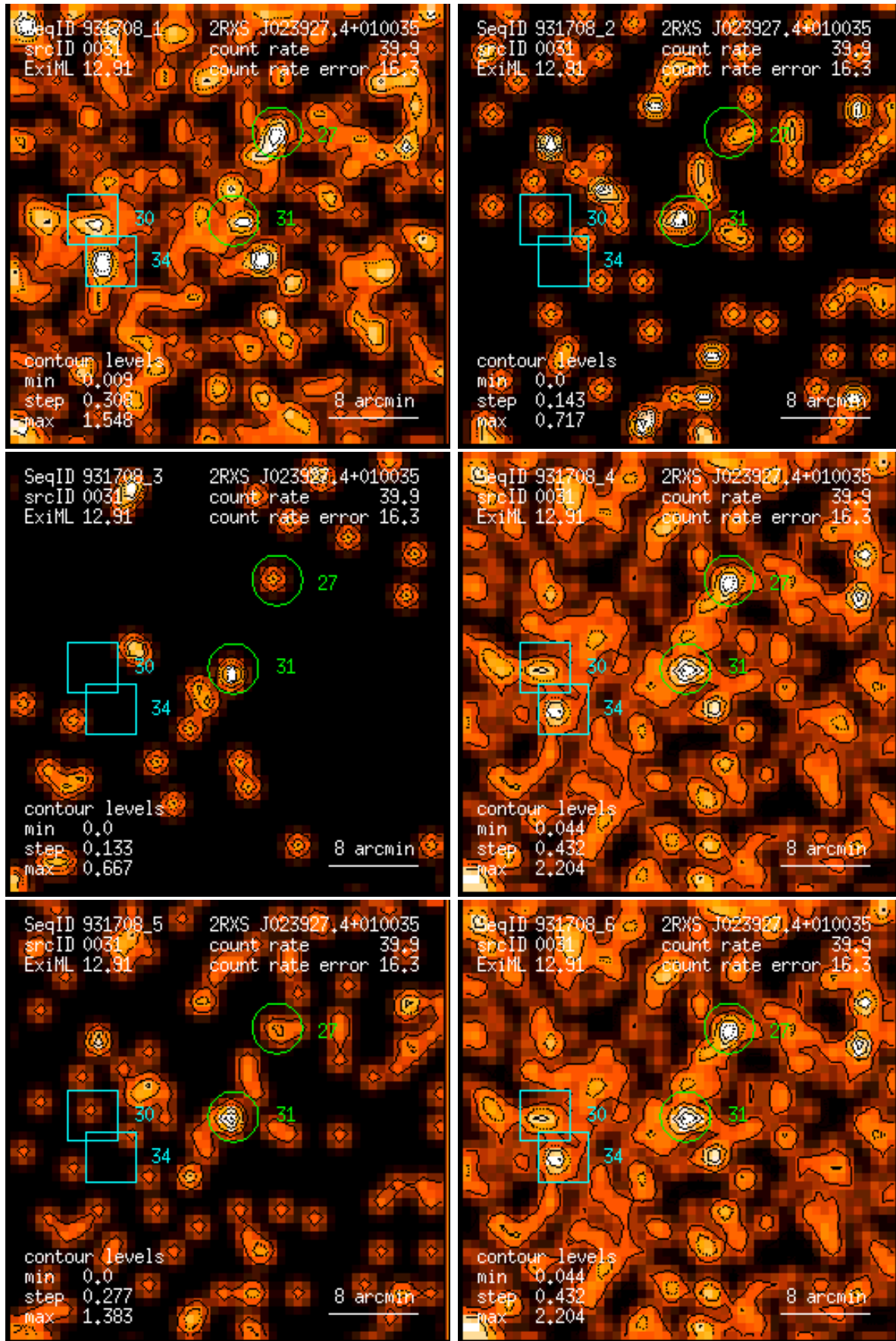
Figure 31: RASS 931708: detection 0031: band rate images, Gaussian filter: (1) PSPC channels 11 – 41, (2) 52 – 90, (3) 91 – 201, (4) 11 – 235, (5) 52 – 201, (6) 11 – 201. Broad band rates in counts/ks. Band rate contour levels in counts/ks/arcmin 2 .
