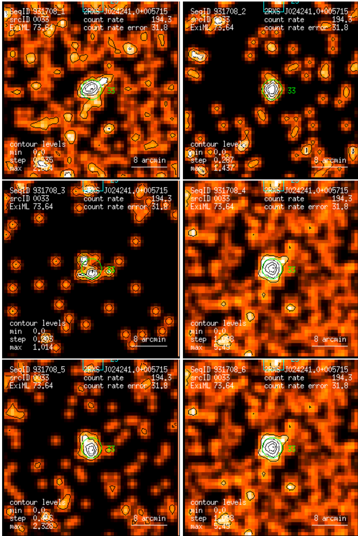
Figure 33: RASS 931708: detection 0033: band rate images, Gaussian filter: (1) PSPC channels 11 – 41, (2) 52 – 90, (3) 91 – 201, (4) 11 – 235, (5) 52 – 201, (6) 11 – 201. Broad band rates in counts/ks. Band rate contour levels in counts/ks/arcmin 2 .
