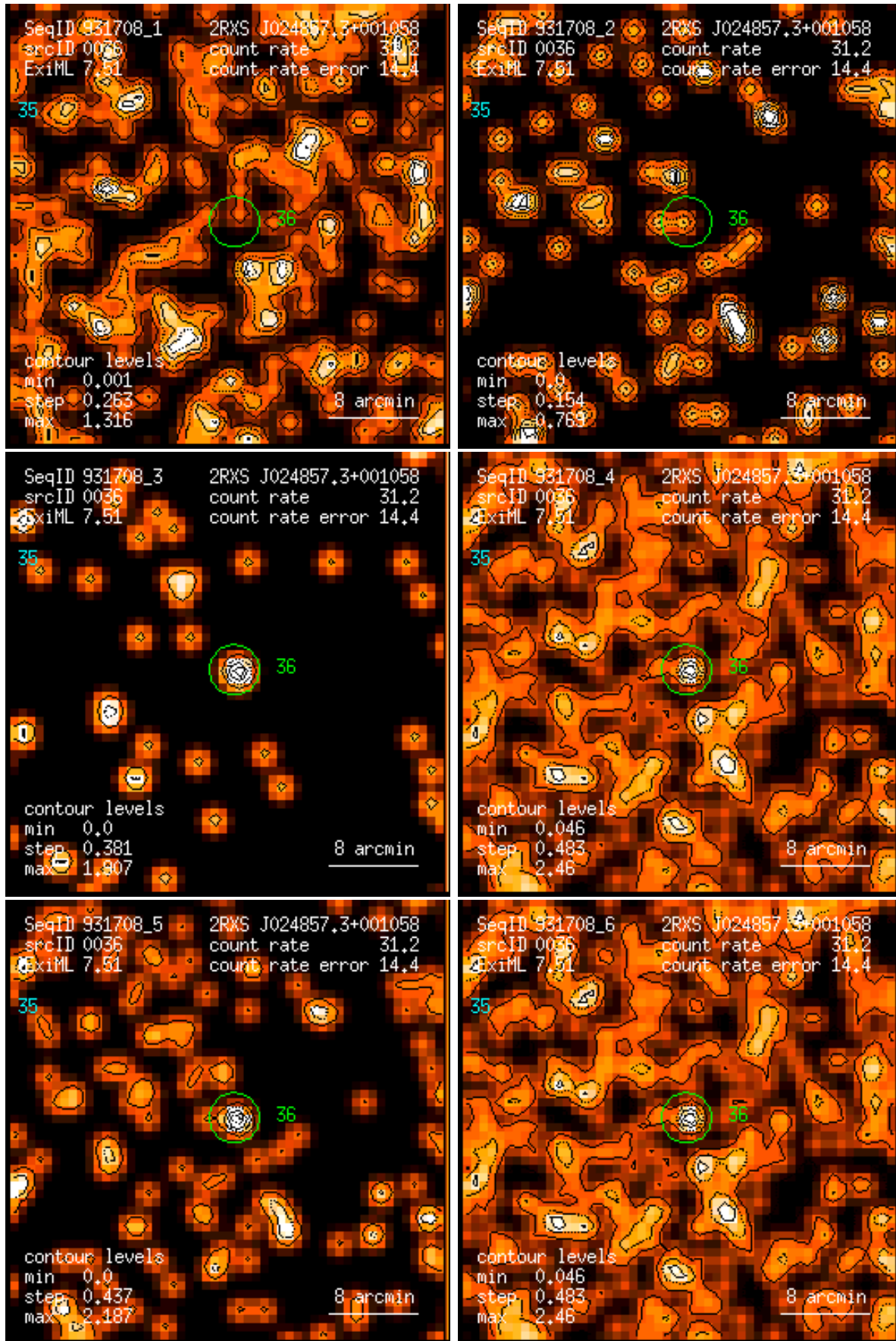
Figure 36: RASS 931708: detection 0036: band rate images, Gaussian filter: (1) PSPC channels 11 – 41, (2) 52 – 90, (3) 91 – 201, (4) 11 – 235, (5) 52 – 201, (6) 11 – 201. Broad band rates in counts/ks. Band rate contour levels in counts/ks/arcmin 2 .
