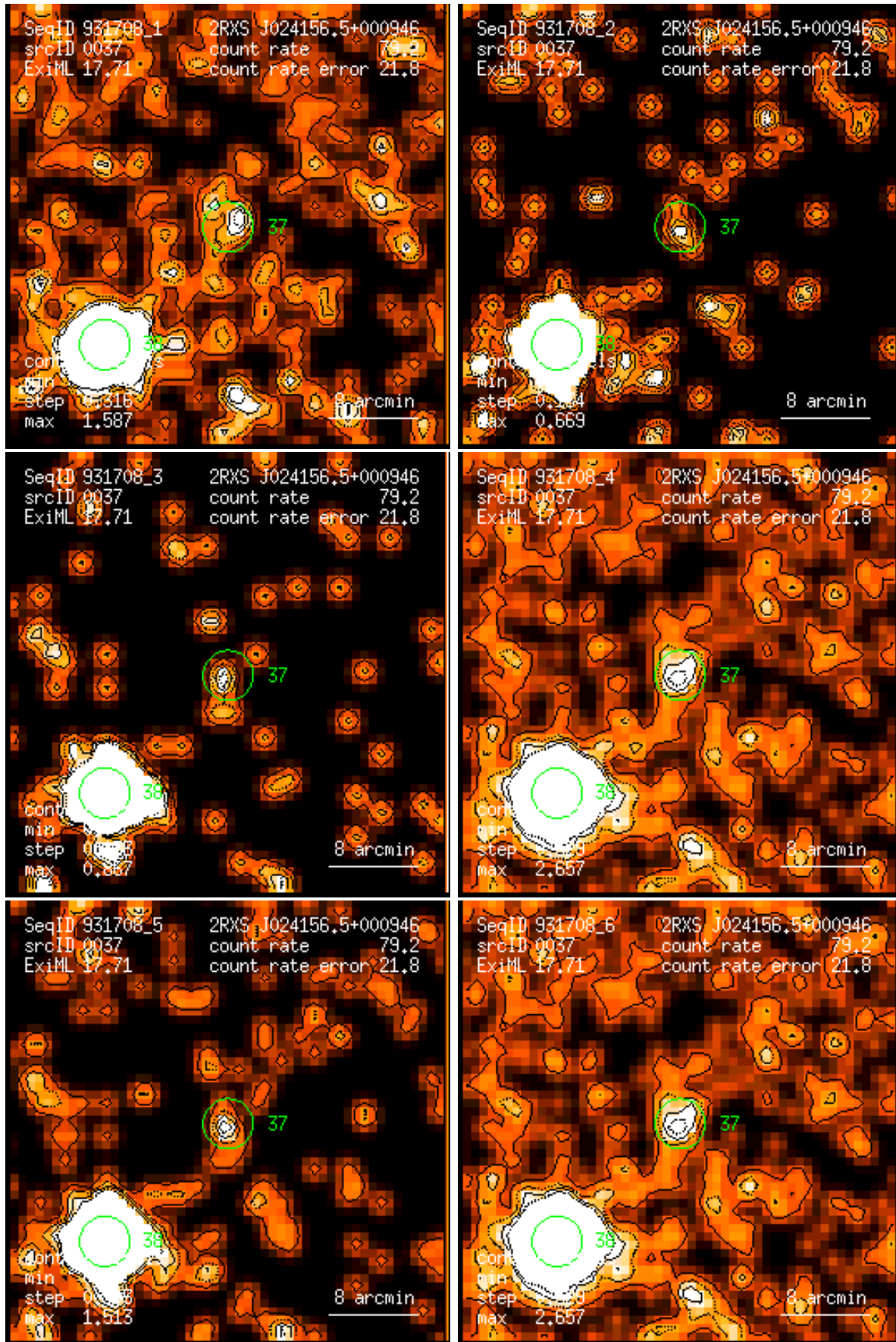
Figure 37: RASS 931708: detection 0037: band rate images, Gaussian filter: (1) PSPC channels 11 – 41, (2) 52 – 90, (3) 91 – 201, (4) 11 – 235, (5) 52 – 201, (6) 11 – 201. Broad band rates in counts/ks. Band rate contour levels in counts/ks/arcmin 2 .
