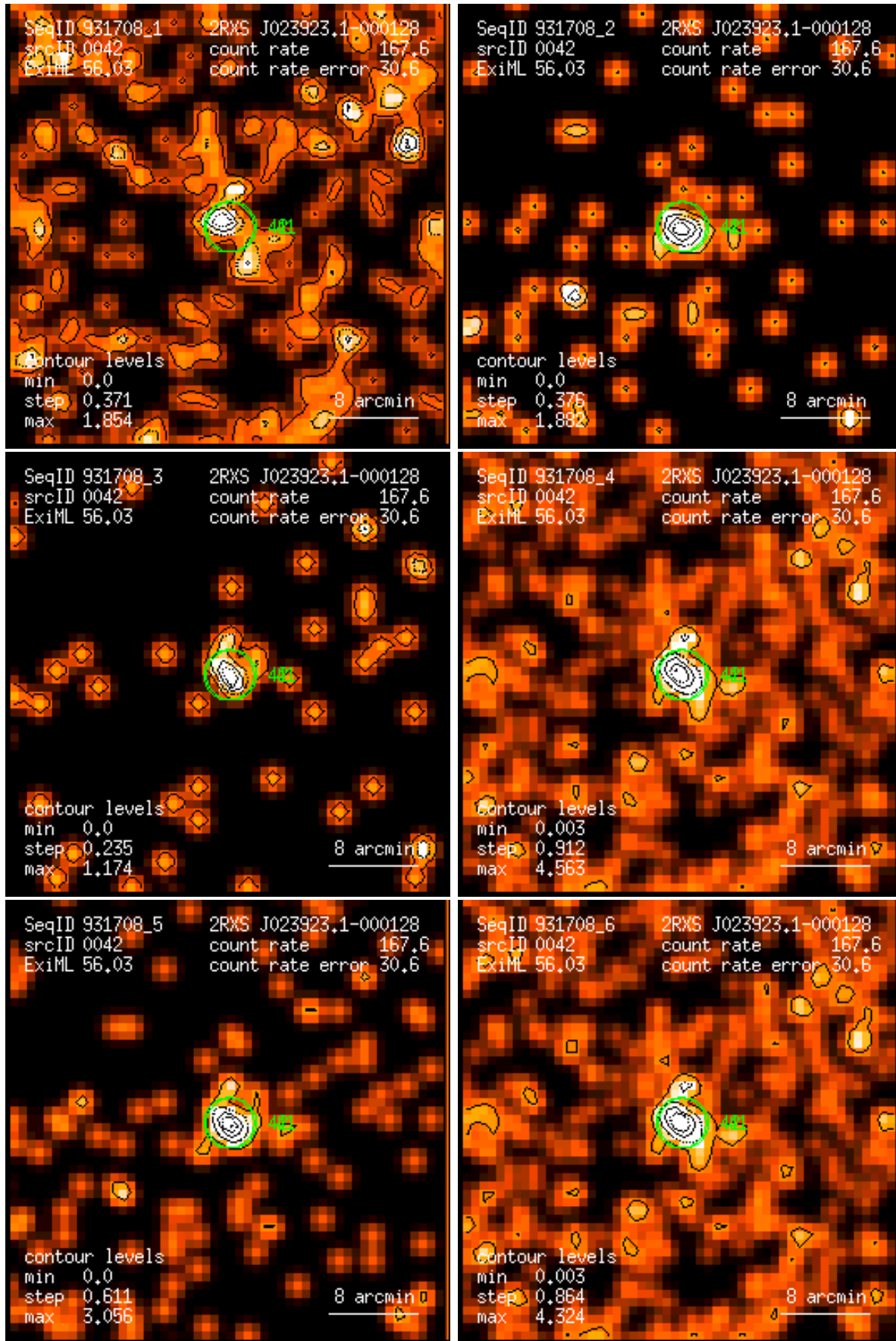
Figure 42: RASS 931708: detection 0042: band rate images, Gaussian filter: (1) PSPC channels 11 – 41, (2) 52 – 90, (3) 91 – 201, (4) 11 – 235, (5) 52 – 201, (6) 11 – 201. Broad band rates in counts/ks. Band rate contour levels in counts/ks/arcmin 2 .
