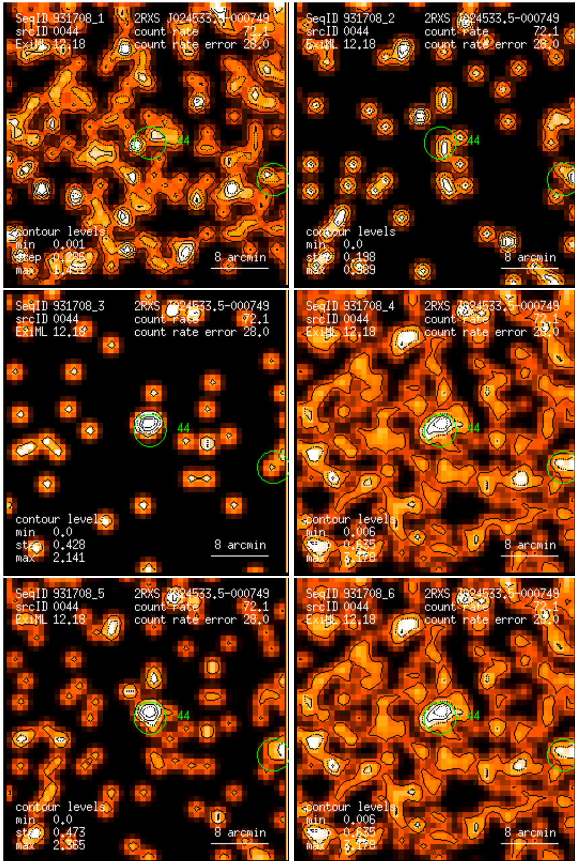
Figure 44: RASS 931708: detection 0044: band rate images, Gaussian filter: (1) PSPC channels 11 – 41, (2) 52 – 90, (3) 91 – 201, (4) 11 – 235, (5) 52 – 201, (6) 11 – 201. Broad band rates in counts/ks. Band rate contour levels in counts/ks/arcmin 2 .
