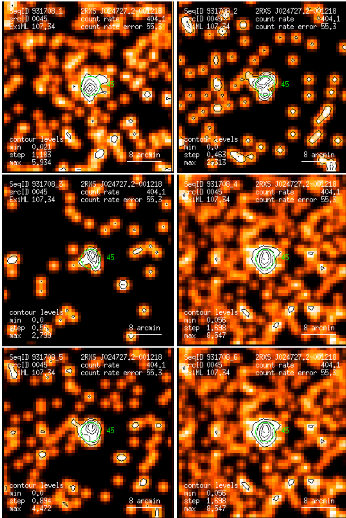
Figure 45: RASS 931708: detection 0045: band rate images, Gaussian filter: (1) PSPC channels 11 – 41, (2) 52 – 90, (3) 91 – 201, (4) 11 – 235, (5) 52 – 201, (6) 11 – 201. Broad band rates in counts/ks. Band rate contour levels in counts/ks/arcmin 2 .
