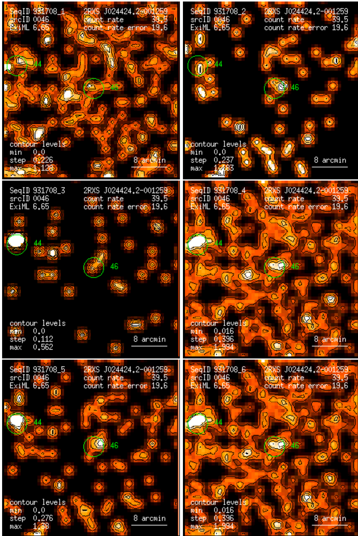
Figure 46: RASS 931708: detection 0046: band rate images, Gaussian filter: (1) PSPC channels 11 – 41, (2) 52 – 90, (3) 91 – 201, (4) 11 – 235, (5) 52 – 201, (6) 11 – 201. Broad band rates in counts/ks. Band rate contour levels in counts/ks/arcmin 2 .
