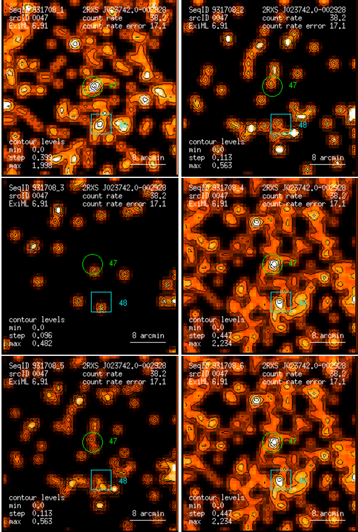
Figure 47: RASS 931708: detection 0047: band rate images, Gaussian filter: (1) PSPC channels 11 – 41, (2) 52 – 90, (3) 91 – 201, (4) 11 – 235, (5) 52 – 201, (6) 11 – 201. Broad band rates in counts/ks. Band rate contour levels in counts/ks/arcmin 2 .
