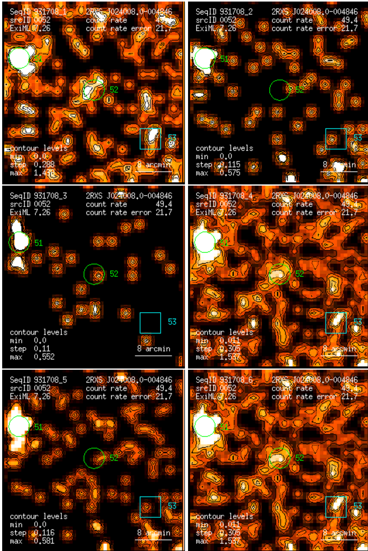
Figure 52: RASS 931708: detection 0052: band rate images, Gaussian filter: (1) PSPC channels 11 – 41, (2) 52 – 90, (3) 91 – 201, (4) 11 – 235, (5) 52 – 201, (6) 11 – 201. Broad band rates in counts/ks. Band rate contour levels in counts/ks/arcmin 2 .
