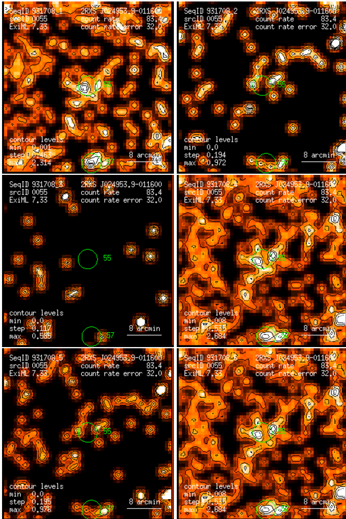
Figure 55: RASS 931708: detection 0055: band rate images, Gaussian filter: (1) PSPC channels 11 – 41, (2) 52 – 90, (3) 91 – 201, (4) 11 – 235, (5) 52 – 201, (6) 11 – 201. Broad band rates in counts/ks. Band rate contour levels in counts/ks/arcmin 2 .
