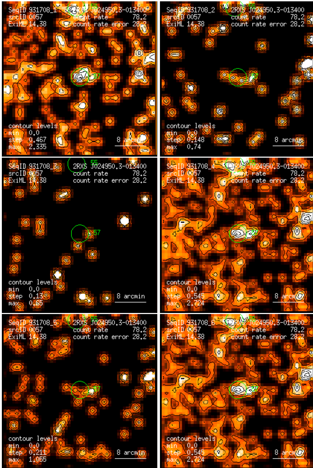
Figure 57: RASS 931708: detection 0057: band rate images, Gaussian filter: (1) PSPC channels 11 – 41, (2) 52 – 90, (3) 91 – 201, (4) 11 – 235, (5) 52 – 201, (6) 11 – 201. Broad band rates in counts/ks. Band rate contour levels in counts/ks/arcmin 2 .
