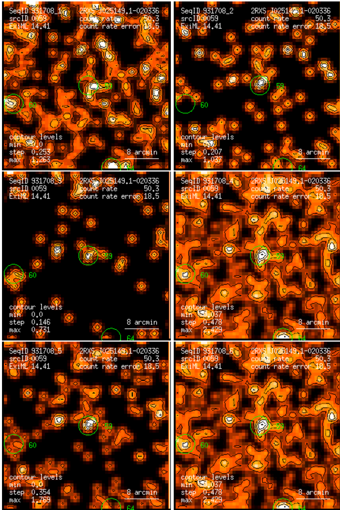
Figure 59: RASS 931708: detection 0059: band rate images, Gaussian filter: (1) PSPC channels 11 – 41, (2) 52 – 90, (3) 91 – 201, (4) 11 – 235, (5) 52 – 201, (6) 11 – 201. Broad band rates in counts/ks. Band rate contour levels in counts/ks/arcmin 2 .
