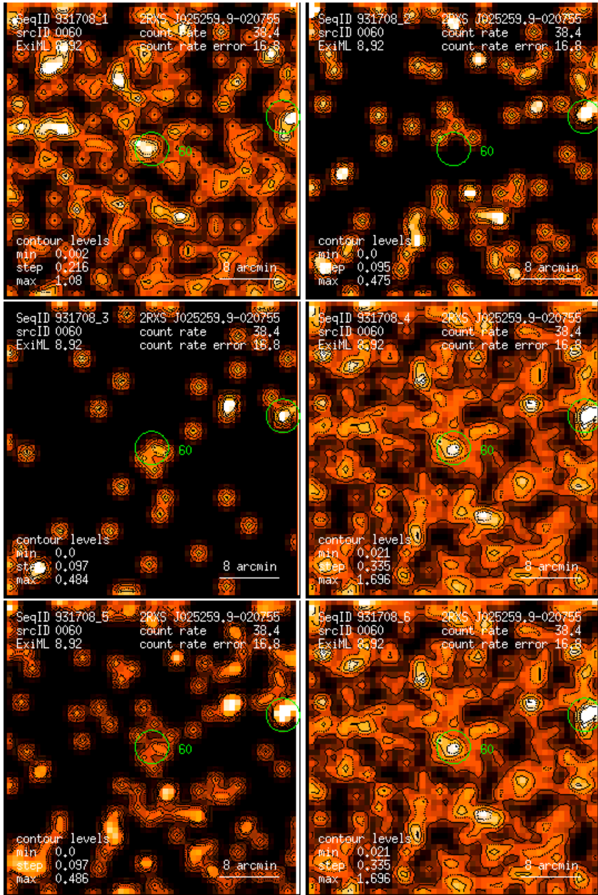
Figure 60: RASS 931708: detection 0060: band rate images, Gaussian filter: (1) PSPC channels 11 – 41, (2) 52 – 90, (3) 91 – 201, (4) 11 – 235, (5) 52 – 201, (6) 11 – 201. Broad band rates in counts/ks. Band rate contour levels in counts/ks/arcmin 2 .
