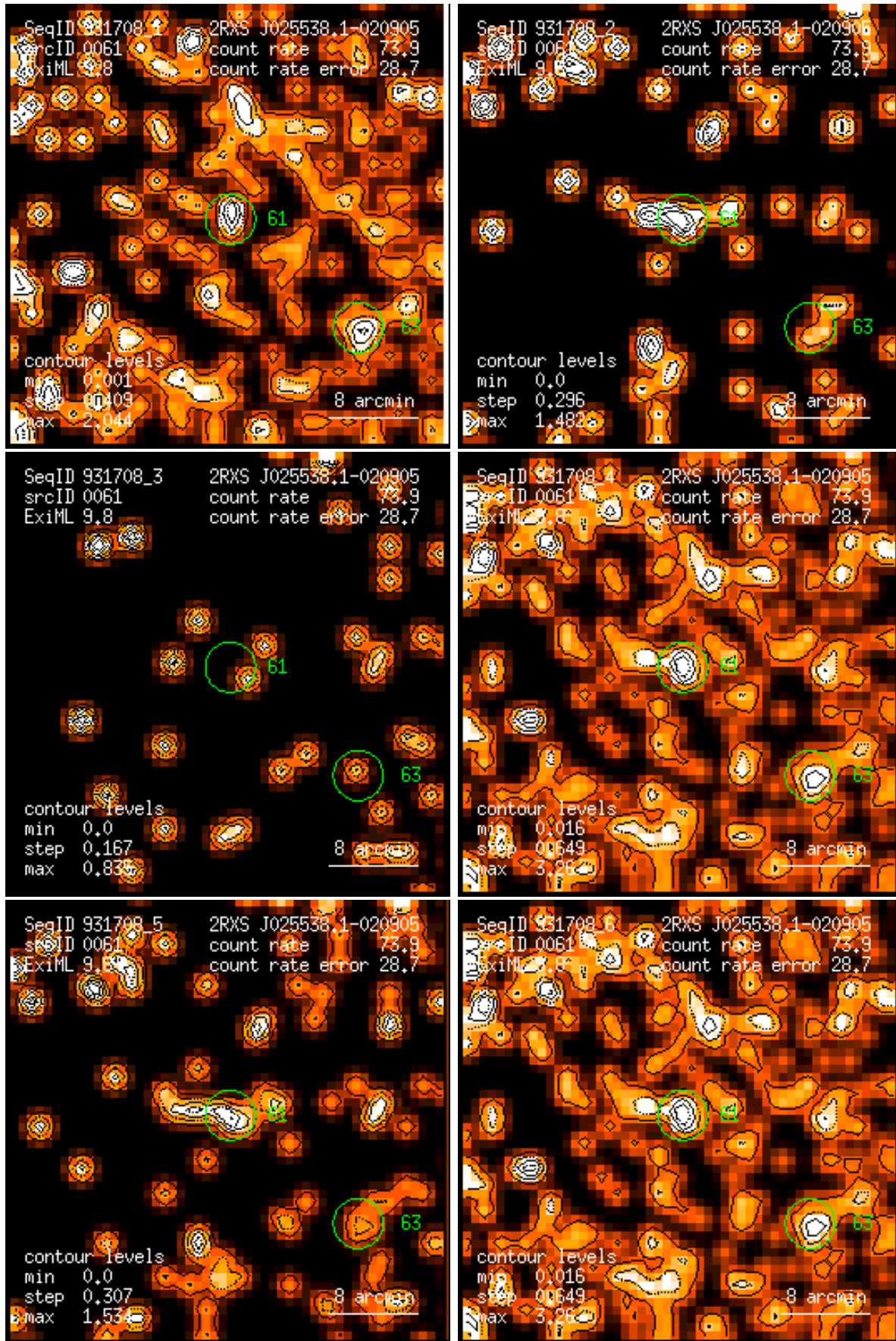
Figure 61: RASS 931708: detection 0061: band rate images, Gaussian filter: (1) PSPC channels 11 – 41, (2) 52 – 90, (3) 91 – 201, (4) 11 – 235, (5) 52 – 201, (6) 11 – 201. Broad band rates in counts/ks. Band rate contour levels in counts/ks/arcmin 2 .
