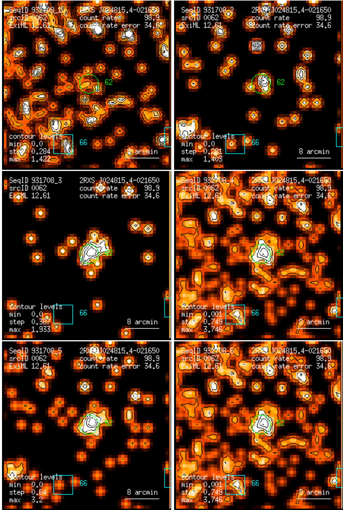
Figure 62: RASS 931708: detection 0062: band rate images, Gaussian filter: (1) PSPC channels 11 – 41, (2) 52 – 90, (3) 91 – 201, (4) 11 – 235, (5) 52 – 201, (6) 11 – 201. Broad band rates in counts/ks. Band rate contour levels in counts/ks/arcmin 2 .
