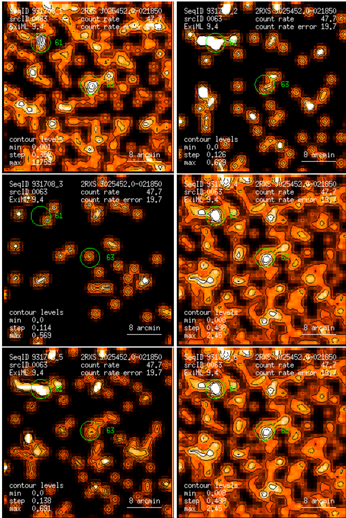
Figure 63: RASS 931708: detection 0063: band rate images, Gaussian filter: (1) PSPC channels 11 – 41, (2) 52 – 90, (3) 91 – 201, (4) 11 – 235, (5) 52 – 201, (6) 11 – 201. Broad band rates in counts/ks. Band rate contour levels in counts/ks/arcmin 2 .
