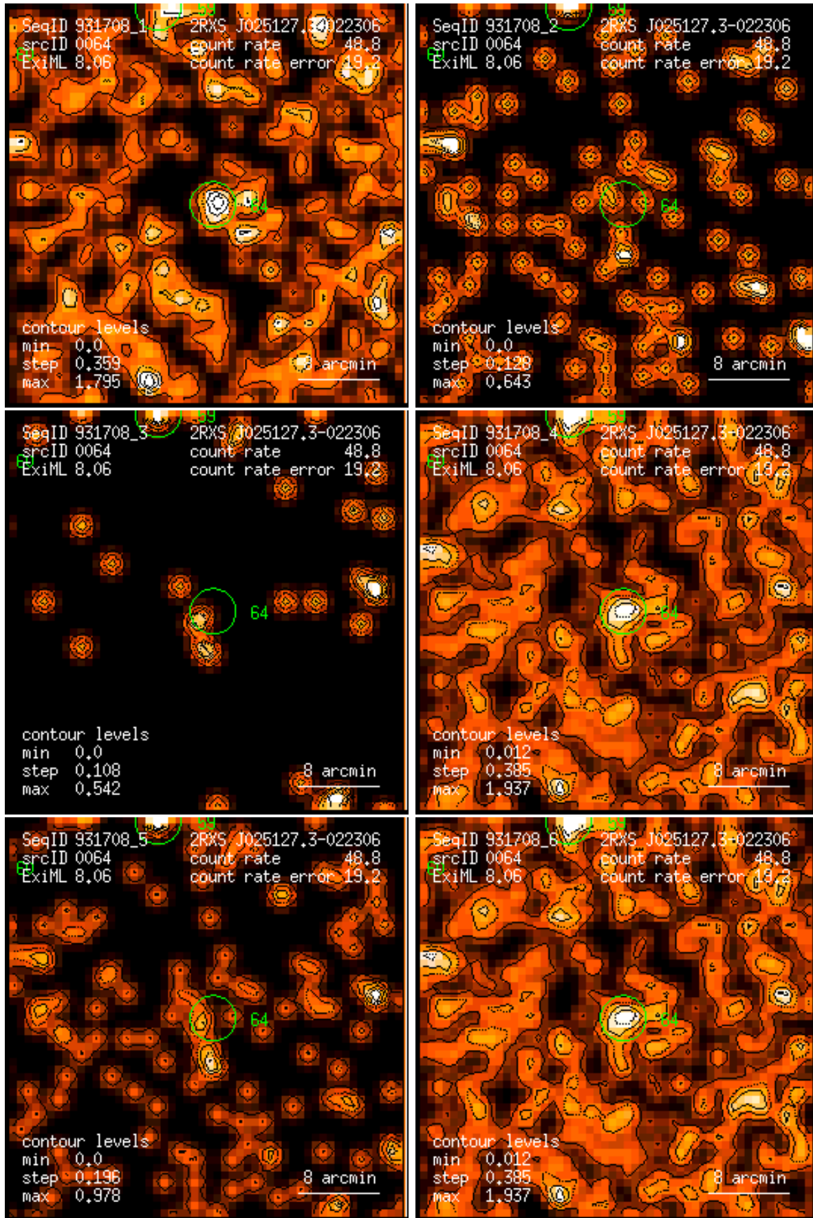
Figure 64: RASS 931708: detection 0064: band rate images, Gaussian filter: (1) PSPC channels 11 – 41, (2) 52 – 90, (3) 91 – 201, (4) 11 – 235, (5) 52 – 201, (6) 11 – 201. Broad band rates in counts/ks. Band rate contour levels in counts/ks/arcmin 2 .
