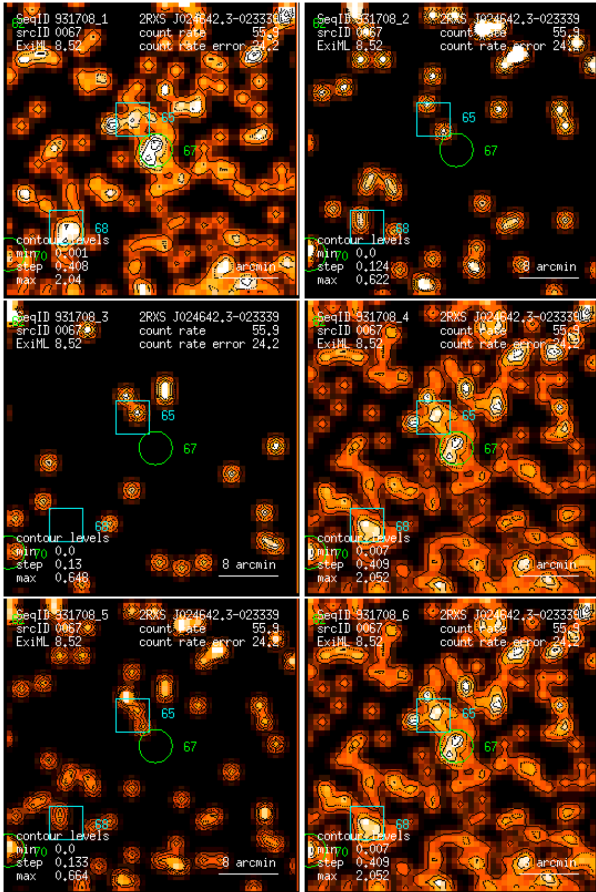
Figure 67: RASS 931708: detection 0067: band rate images, Gaussian filter: (1) PSPC channels 11 – 41, (2) 52 – 90, (3) 91 – 201, (4) 11 – 235, (5) 52 – 201, (6) 11 – 201. Broad band rates in counts/ks. Band rate contour levels in counts/ks/arcmin 2 .
