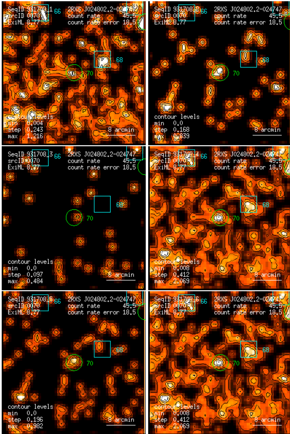
Figure 70: RASS 931708: detection 0070: band rate images, Gaussian filter: (1) PSPC channels 11 – 41, (2) 52 – 90, (3) 91 – 201, (4) 11 – 235, (5) 52 – 201, (6) 11 – 201. Broad band rates in counts/ks. Band rate contour levels in counts/ks/arcmin 2 .
