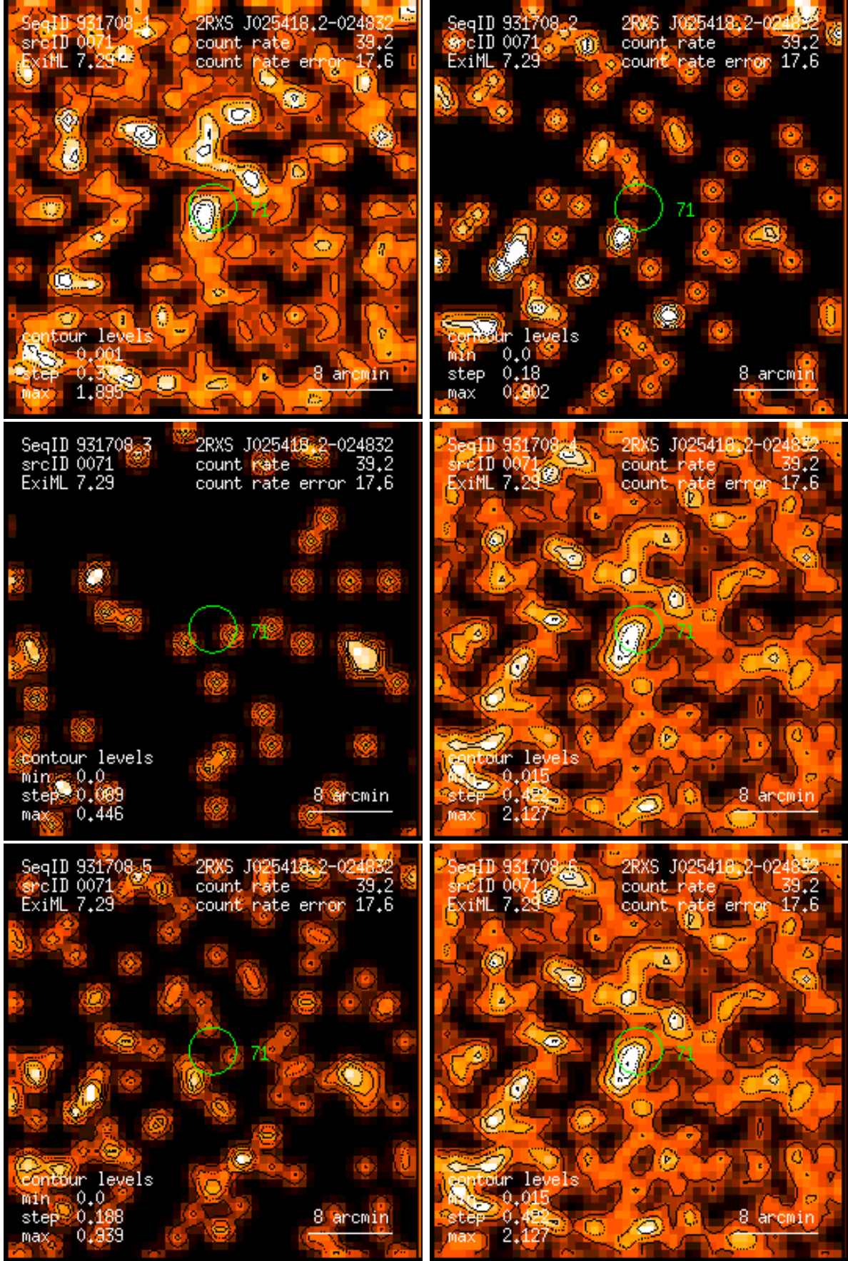
Figure 71: RASS 931708: detection 0071: band rate images, Gaussian filter: (1) PSPC channels 11 – 41, (2) 52 – 90, (3) 91 – 201, (4) 11 – 235, (5) 52 – 201, (6) 11 – 201. Broad band rates in counts/ks. Band rate contour levels in counts/ks/arcmin 2 .
