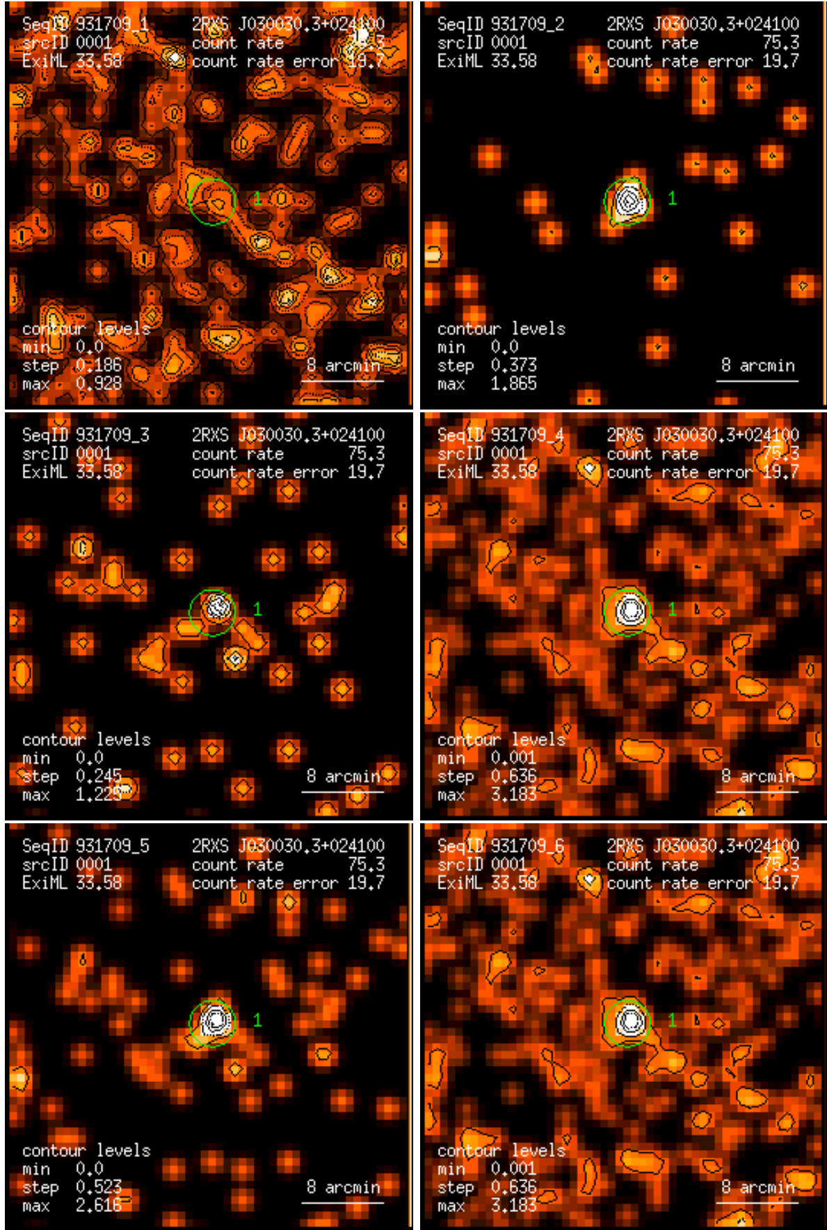
Figure 1: RASS 931709: detection 0001: band rate images, Gaussian filter: (1) PSPC channels 11 – 41, (2) 52 – 90, (3) 91 – 201, (4) 11 – 235, (5) 52 – 201, (6) 11 – 201. Broad band rates in counts/ks. Band rate contour levels in counts/ks/arcmin 2 .
