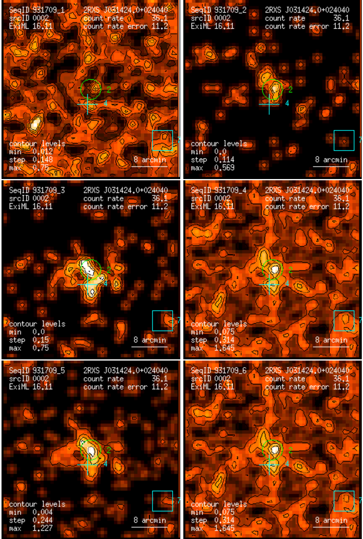
Figure 2: RASS 931709: detection 0002: band rate images, Gaussian filter: (1) PSPC channels 11 – 41, (2) 52 – 90, (3) 91 – 201, (4) 11 – 235, (5) 52 – 201, (6) 11 – 201. Broad band rates in counts/ks. Band rate contour levels in counts/ks/arcmin 2 .
