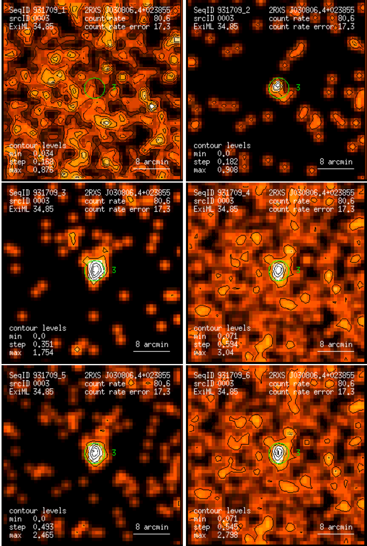
Figure 3: RASS 931709: detection 0003: band rate images, Gaussian filter: (1) PSPC channels 11 – 41, (2) 52 – 90, (3) 91 – 201, (4) 11 – 235, (5) 52 – 201, (6) 11 – 201. Broad band rates in counts/ks. Band rate contour levels in counts/ks/arcmin 2 .
