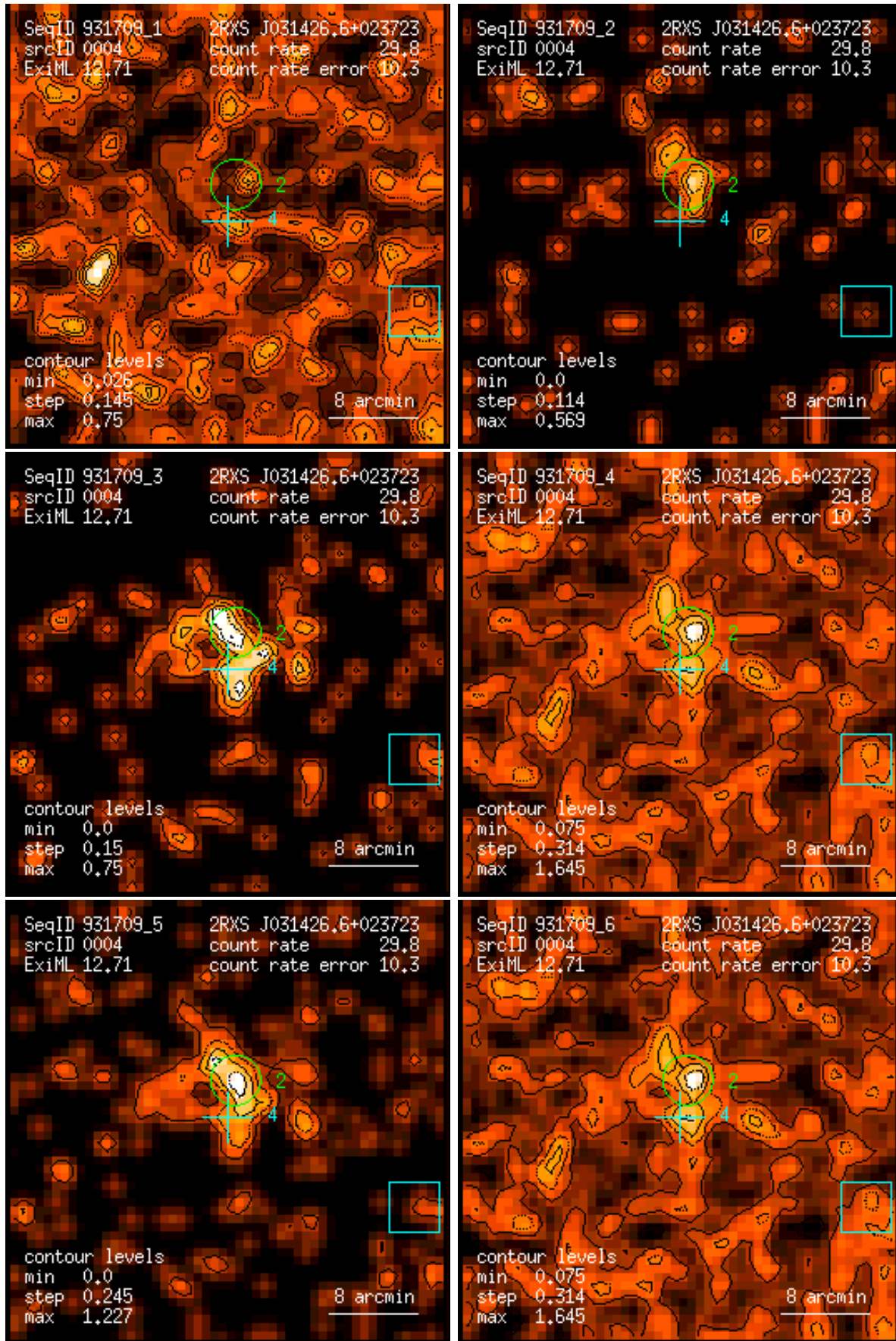
Figure 4: RASS 931709: detection 0004: band rate images, Gaussian filter: (1) PSPC channels 11 – 41, (2) 52 – 90, (3) 91 – 201, (4) 11 – 235, (5) 52 – 201, (6) 11 – 201. Broad band rates in counts/ks. Band rate contour levels in counts/ks/arcmin 2 .
