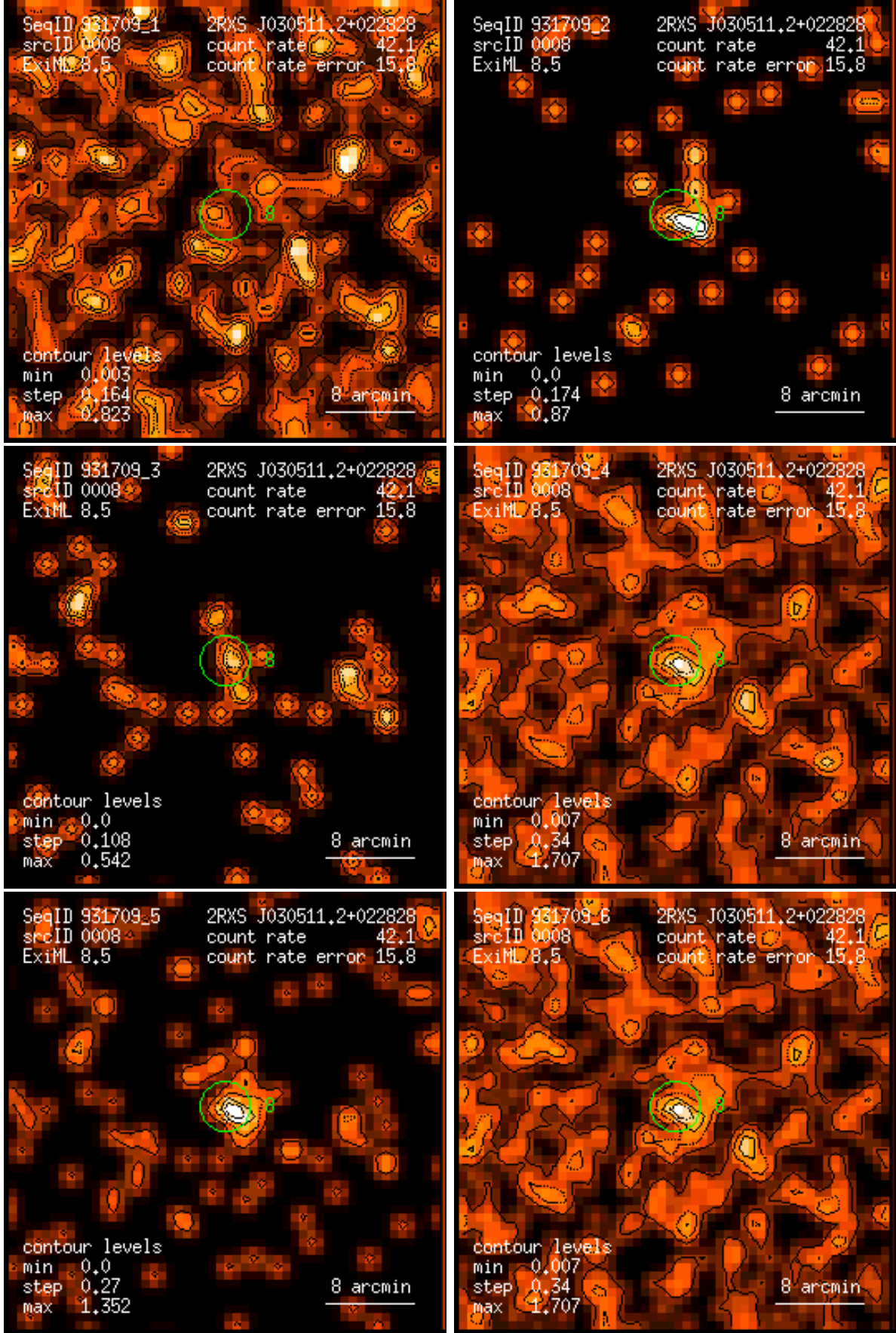
Figure 8: RASS 931709: detection 0008: band rate images, Gaussian filter: (1) PSPC channels 11 – 41, (2) 52 – 90, (3) 91 – 201, (4) 11 – 235, (5) 52 – 201, (6) 11 – 201. Broad band rates in counts/ks. Band rate contour levels in counts/ks/arcmin 2 .
