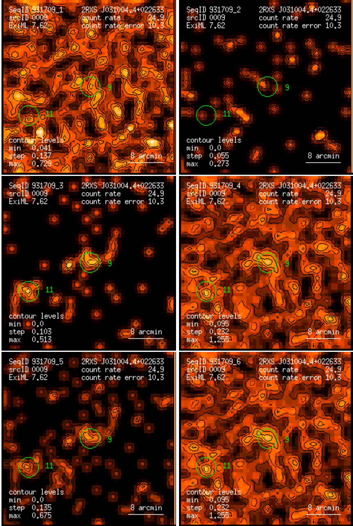
Figure 9: RASS 931709: detection 0009: band rate images, Gaussian filter: (1) PSPC channels 11 – 41, (2) 52 – 90, (3) 91 – 201, (4) 11 – 235, (5) 52 – 201, (6) 11 – 201. Broad band rates in counts/ks. Band rate contour levels in counts/ks/arcmin 2 .
