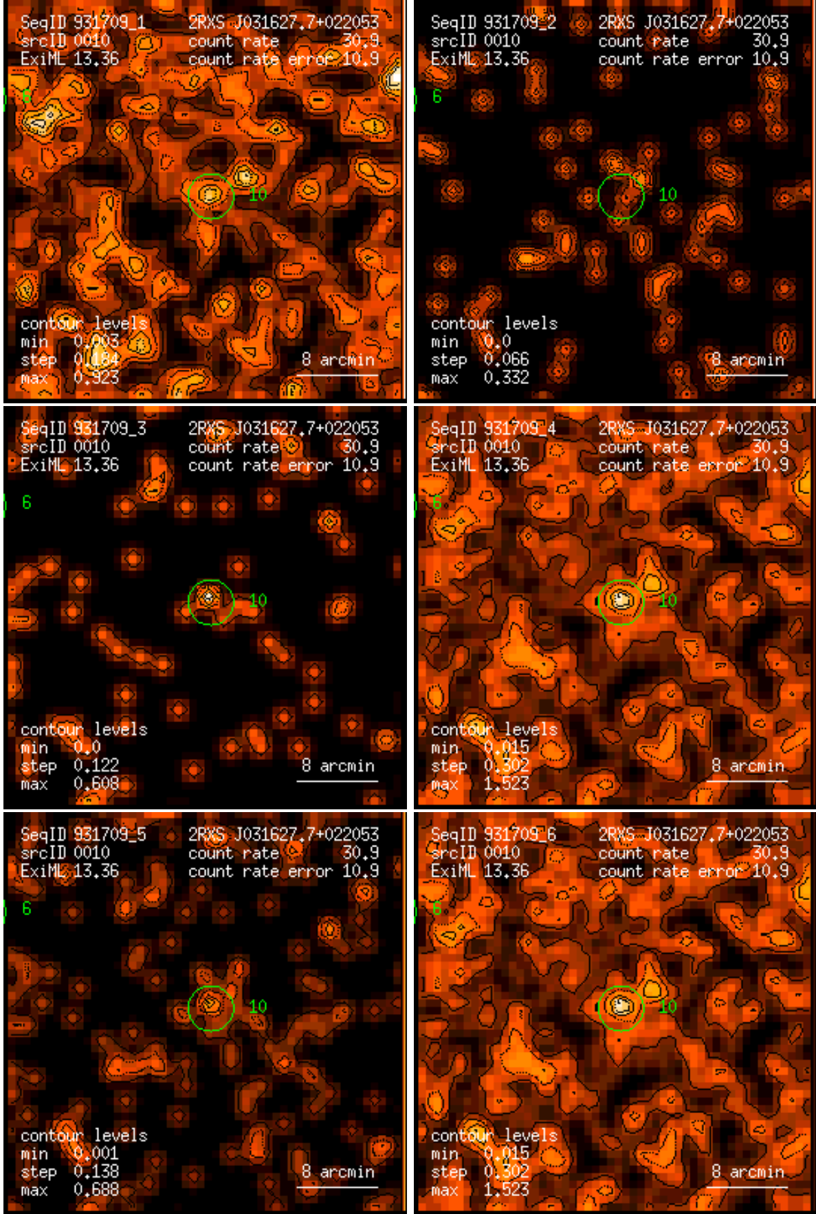
Figure 10: RASS 931709: detection 0010: band rate images, Gaussian filter: (1) PSPC channels 11 – 41, (2) 52 – 90, (3) 91 – 201, (4) 11 – 235, (5) 52 – 201, (6) 11 – 201. Broad band rates in counts/ks. Band rate contour levels in counts/ks/arcmin 2 .
