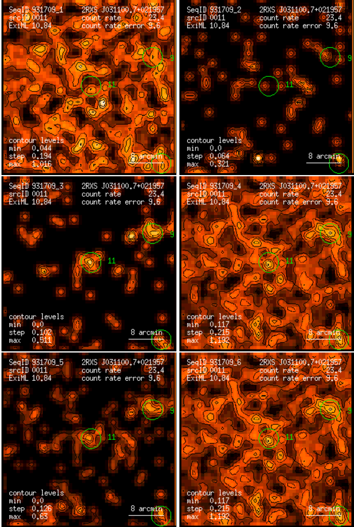
Figure 11: RASS 931709: detection 0011: band rate images, Gaussian filter: (1) PSPC channels 11 – 41, (2) 52 – 90, (3) 91 – 201, (4) 11 – 235, (5) 52 – 201, (6) 11 – 201. Broad band rates in counts/ks. Band rate contour levels in counts/ks/arcmin 2 .
