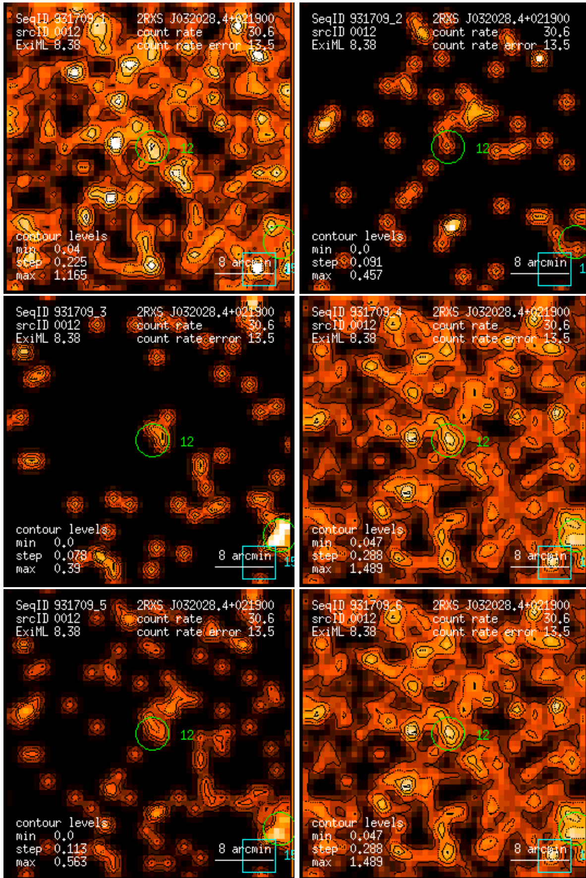
Figure 12: RASS 931709: detection 0012: band rate images, Gaussian filter: (1) PSPC channels 11 – 41, (2) 52 – 90, (3) 91 – 201, (4) 11 – 235, (5) 52 – 201, (6) 11 – 201. Broad band rates in counts/ks. Band rate contour levels in counts/ks/arcmin 2 .
