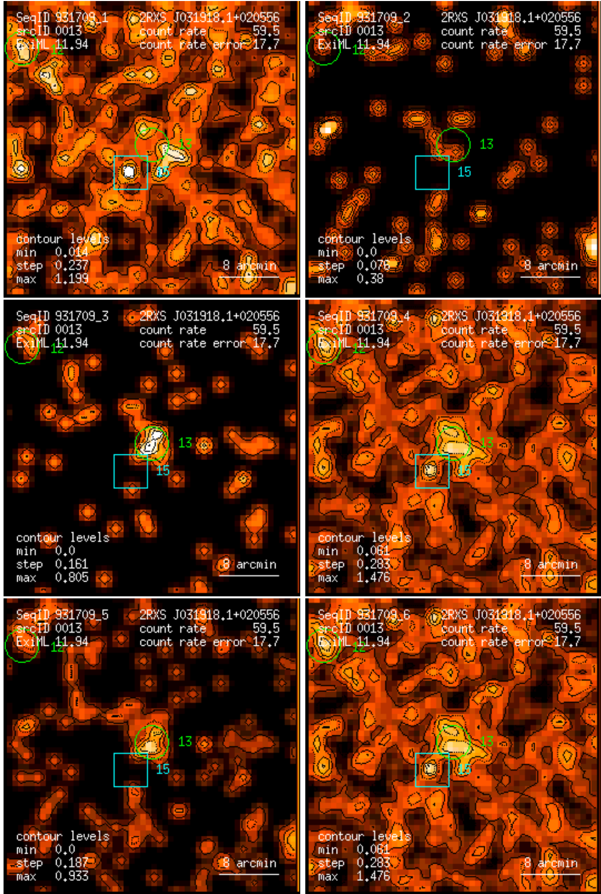
Figure 13: RASS 931709: detection 0013: band rate images, Gaussian filter: (1) PSPC channels 11 – 41, (2) 52 – 90, (3) 91 – 201, (4) 11 – 235, (5) 52 – 201, (6) 11 – 201. Broad band rates in counts/ks. Band rate contour levels in counts/ks/arcmin 2 .
