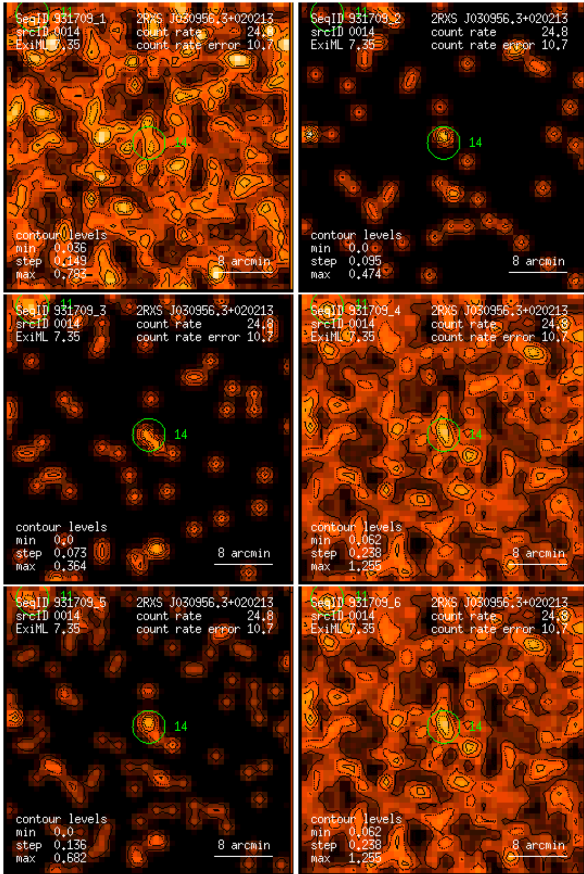
Figure 14: RASS 931709: detection 0014: band rate images, Gaussian filter: (1) PSPC channels 11 – 41, (2) 52 – 90, (3) 91 – 201, (4) 11 – 235, (5) 52 – 201, (6) 11 – 201. Broad band rates in counts/ks. Band rate contour levels in counts/ks/arcmin 2 .
