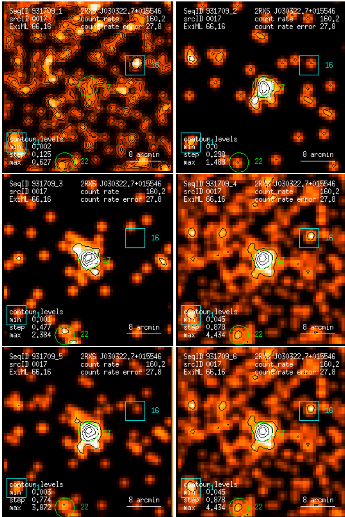
Figure 17: RASS 931709: detection 0017: band rate images, Gaussian filter: (1) PSPC channels 11 – 41, (2) 52 – 90, (3) 91 – 201, (4) 11 – 235, (5) 52 – 201, (6) 11 – 201. Broad band rates in counts/ks. Band rate contour levels in counts/ks/arcmin 2 .
