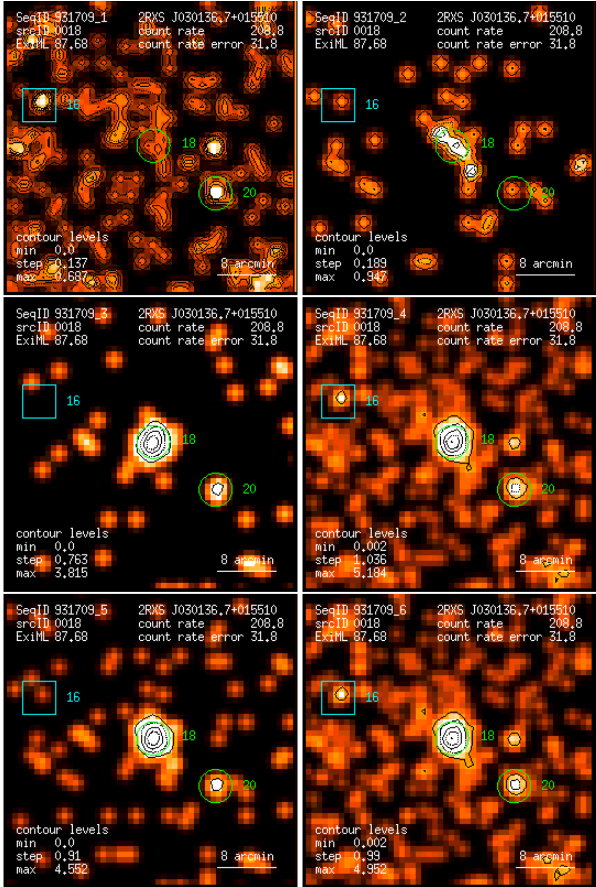
Figure 18: RASS 931709: detection 0018: band rate images, Gaussian filter: (1) PSPC channels 11 – 41, (2) 52 – 90, (3) 91 – 201, (4) 11 – 235, (5) 52 – 201, (6) 11 – 201. Broad band rates in counts/ks. Band rate contour levels in counts/ks/arcmin 2 .
