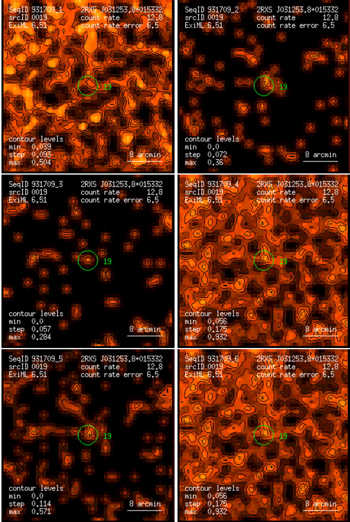
Figure 19: RASS 931709: detection 0019: band rate images, Gaussian filter: (1) PSPC channels 11 – 41, (2) 52 – 90, (3) 91 – 201, (4) 11 – 235, (5) 52 – 201, (6) 11 – 201. Broad band rates in counts/ks. Band rate contour levels in counts/ks/arcmin 2 .
