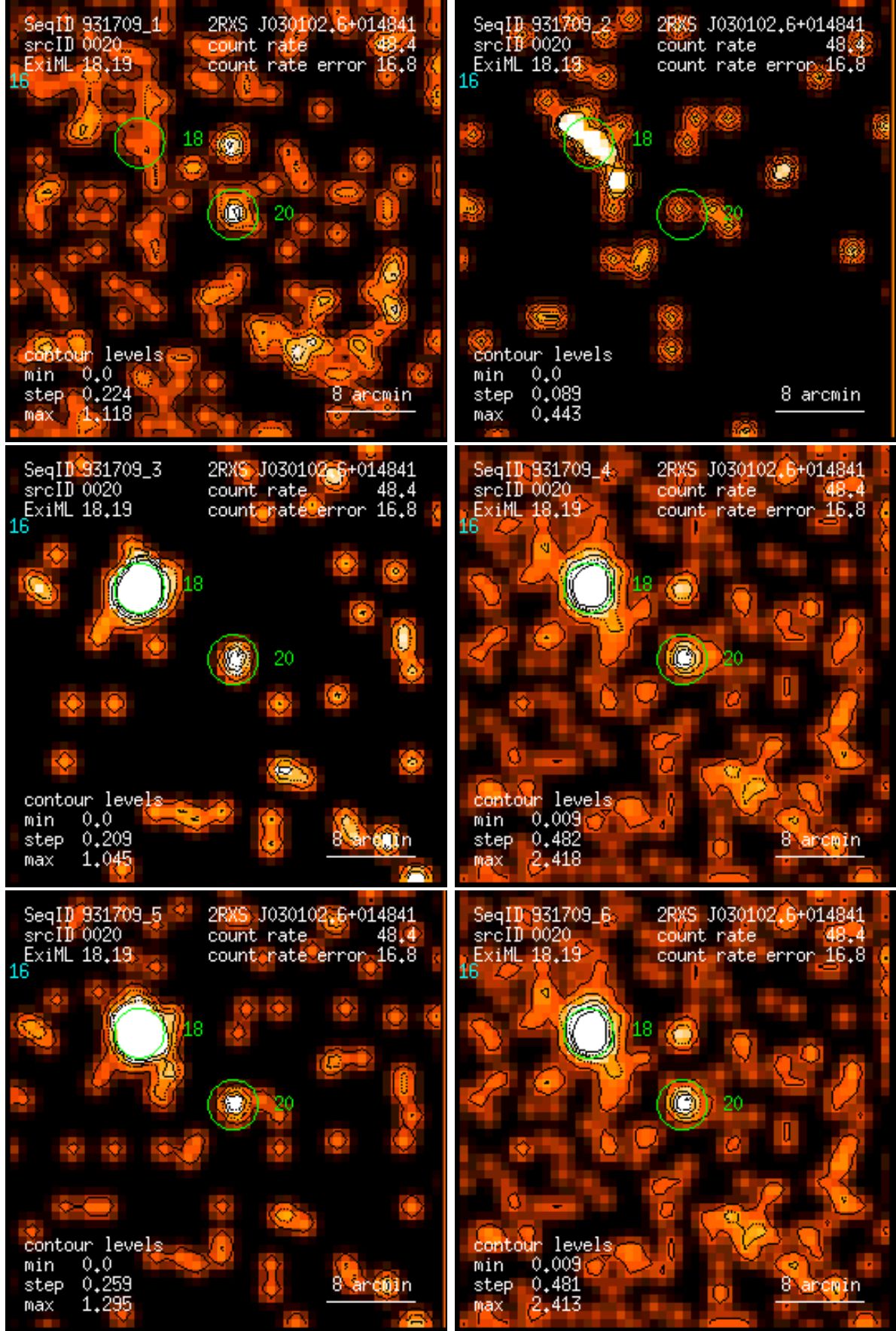
Figure 20: RASS 931709: detection 0020: band rate images, Gaussian filter: (1) PSPC channels 11 – 41, (2) 52 – 90, (3) 91 – 201, (4) 11 – 235, (5) 52 – 201, (6) 11 – 201. Broad band rates in counts/ks. Band rate contour levels in counts/ks/arcmin 2 .
