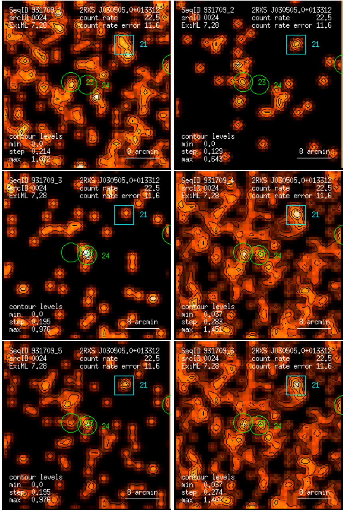
Figure 24: RASS 931709: detection 0024: band rate images, Gaussian filter: (1) PSPC channels 11 – 41, (2) 52 – 90, (3) 91 – 201, (4) 11 – 235, (5) 52 – 201, (6) 11 – 201. Broad band rates in counts/ks. Band rate contour levels in counts/ks/arcmin 2 .
