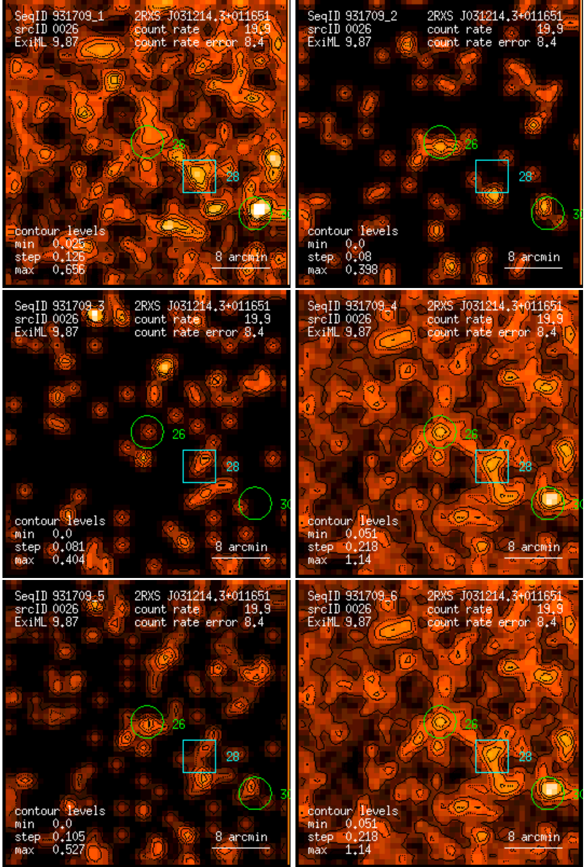
Figure 26: RASS 931709: detection 0026: band rate images, Gaussian filter: (1) PSPC channels 11 – 41, (2) 52 – 90, (3) 91 – 201, (4) 11 – 235, (5) 52 – 201, (6) 11 – 201. Broad band rates in counts/ks. Band rate contour levels in counts/ks/arcmin 2 .
