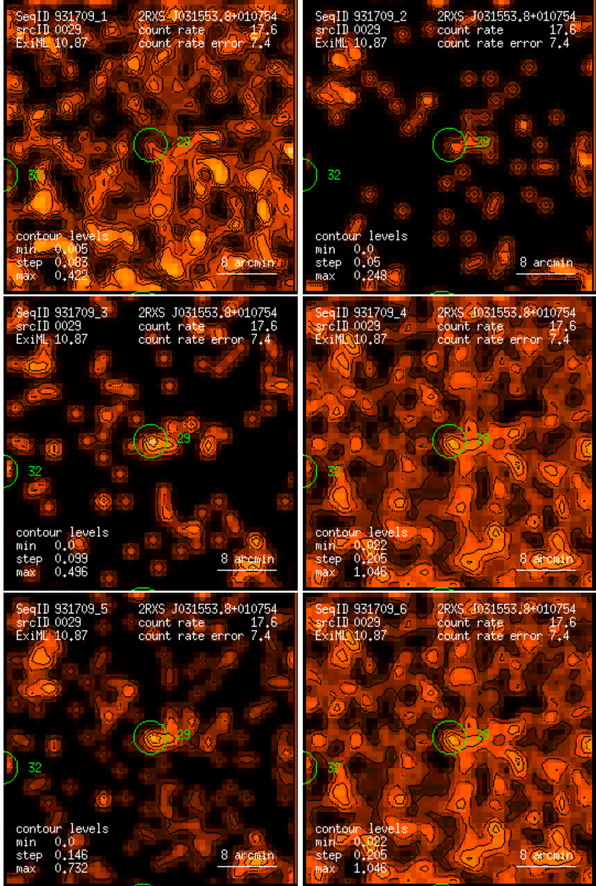
Figure 29: RASS 931709: detection 0029: band rate images, Gaussian filter: (1) PSPC channels 11 – 41, (2) 52 – 90, (3) 91 – 201, (4) 11 – 235, (5) 52 – 201, (6) 11 – 201. Broad band rates in counts/ks. Band rate contour levels in counts/ks/arcmin 2 .
