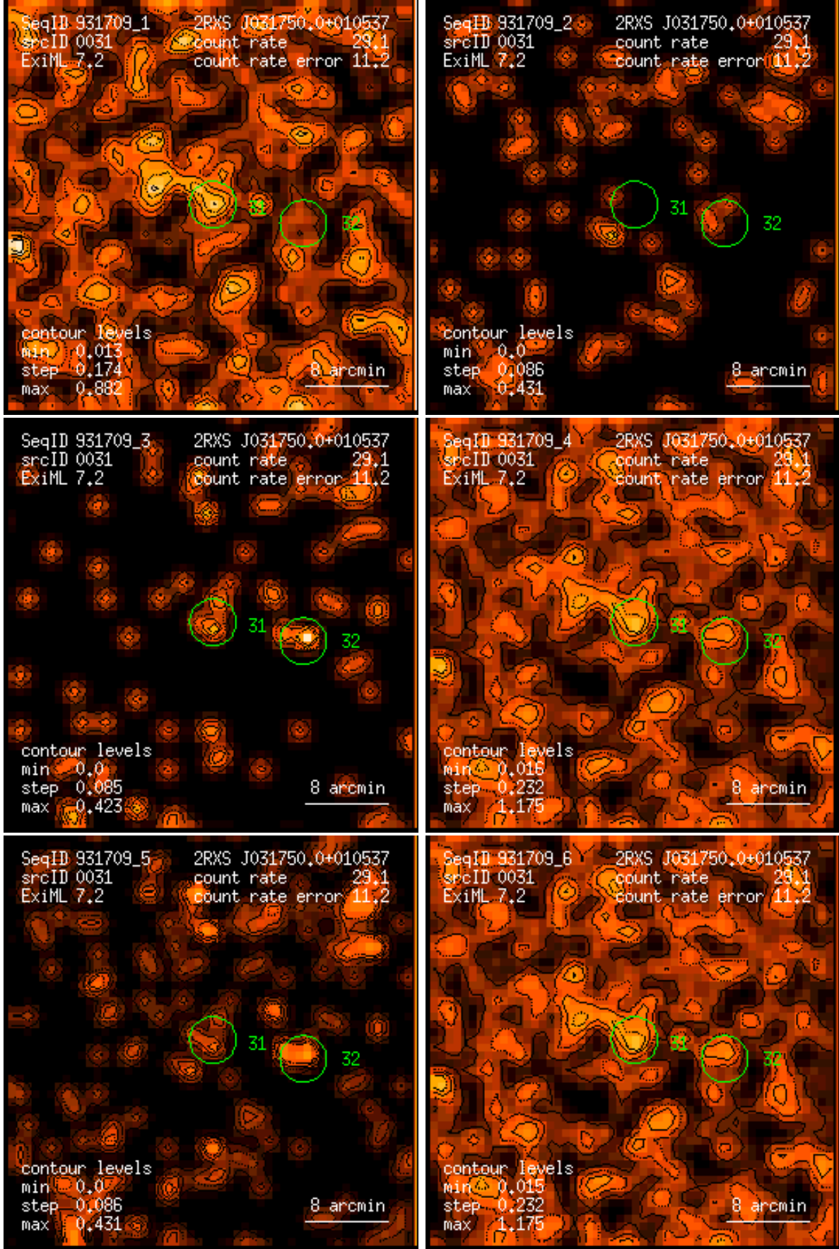
Figure 31: RASS 931709: detection 0031: band rate images, Gaussian filter: (1) PSPC channels 11 – 41, (2) 52 – 90, (3) 91 – 201, (4) 11 – 235, (5) 52 – 201, (6) 11 – 201. Broad band rates in counts/ks. Band rate contour levels in counts/ks/arcmin 2 .
