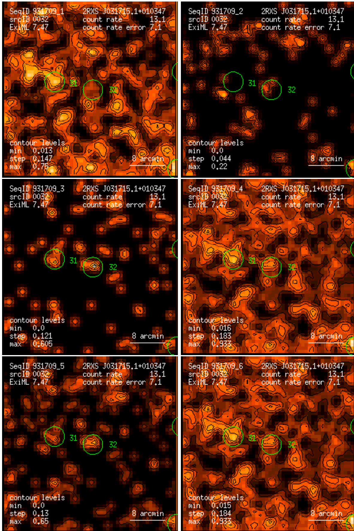
Figure 32: RASS 931709: detection 0032: band rate images, Gaussian filter: (1) PSPC channels 11 – 41, (2) 52 – 90, (3) 91 – 201, (4) 11 – 235, (5) 52 – 201, (6) 11 – 201. Broad band rates in counts/ks. Band rate contour levels in counts/ks/arcmin 2 .
